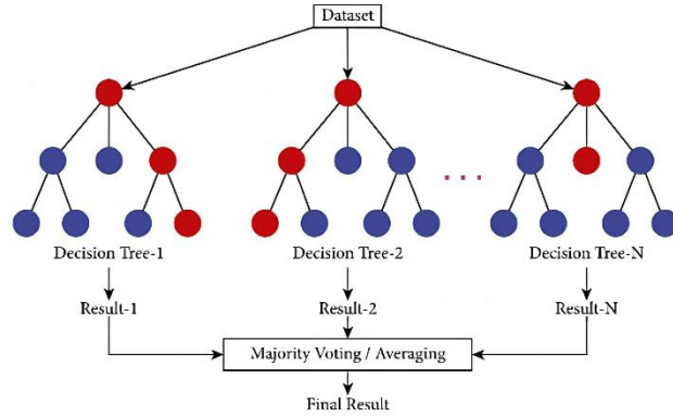
Figure 2. Diagram of a random forest classifier (Khan et al., 2021)
