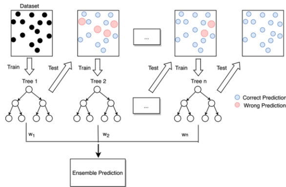
Figure 3. Boosting algorithm (Zhang et al., 2021)
