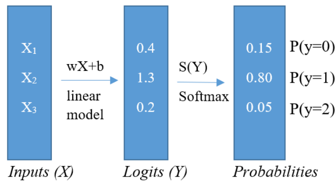
Figure 7. Multinomial logistic classifier
